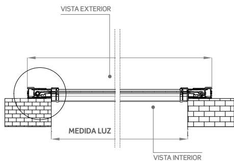
APL. REVERSE (FIG. 2)
