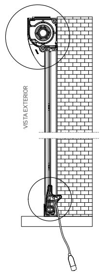
APL. REVERSE (FIG. 2)
